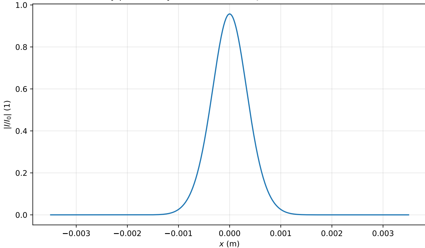
Intensity profile I(x, y = 0, z = 0.876m)/I_0 , \text{Pin}=0.3\text{Pcr} , artificial time
